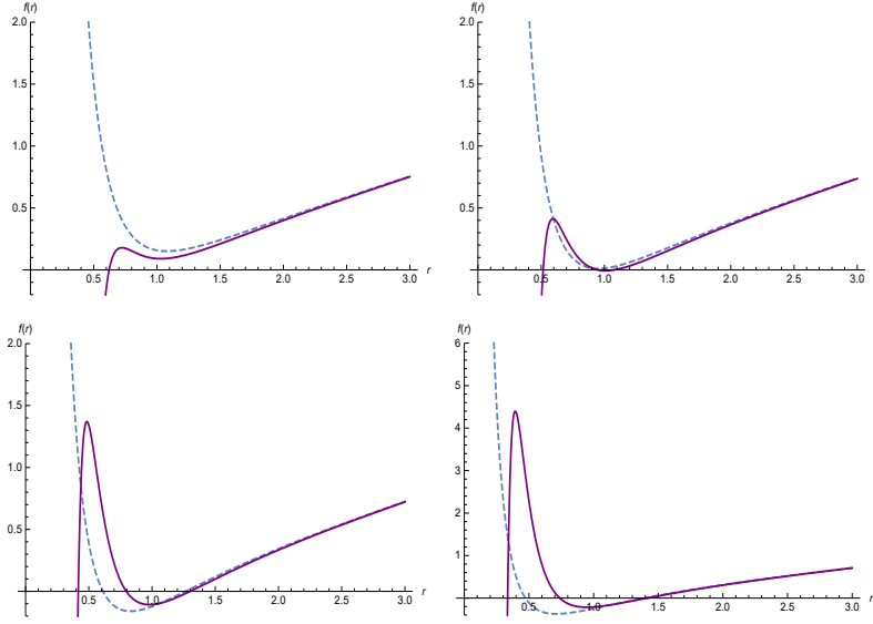
Figure 1: f(r) versus of r with different p for the \alpha' corrected Reissner-Nordström AdS black hole. Plots have been depicted with p = 1.5, 1.4, 1.3, 1.2 from left to right. Dashed line shows the Reissner-Nordström black hole without correction ( \alpha' = 0 ). As p decreases, two separated horizons are created. There exists critical p for which we have one coincidence horizon. Plots have been depicted with M = 1, \alpha' = M^2(a = 1), \Lambda = -0.1 .
