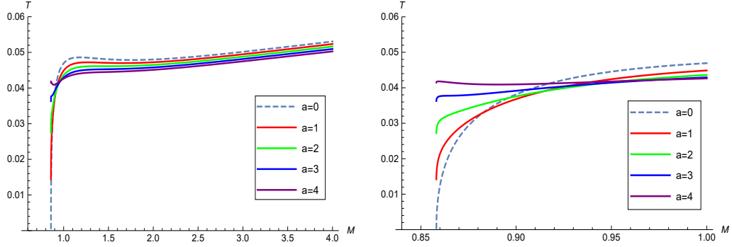
Figure 5: The behavior of temperature versus the mass for the \alpha' corrected Reissner-Nordström AdS black hole. Plots have been depicted with a = 0, 1, 2, 3, 4 ( \alpha' = aM^2 ) and \Lambda = -0.1 while p < p_{cri} .
