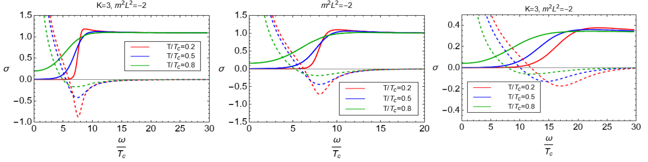
Figure 2. The conductivity of a s -wave holographic superconductor versus \omega/T_c for three different values of \alpha = -0.1 (left panel), 0 (middle panel) and 1/3 (right panel). The solid and dashed curves show the real and imaginary parts of the conductivity, respectively.
