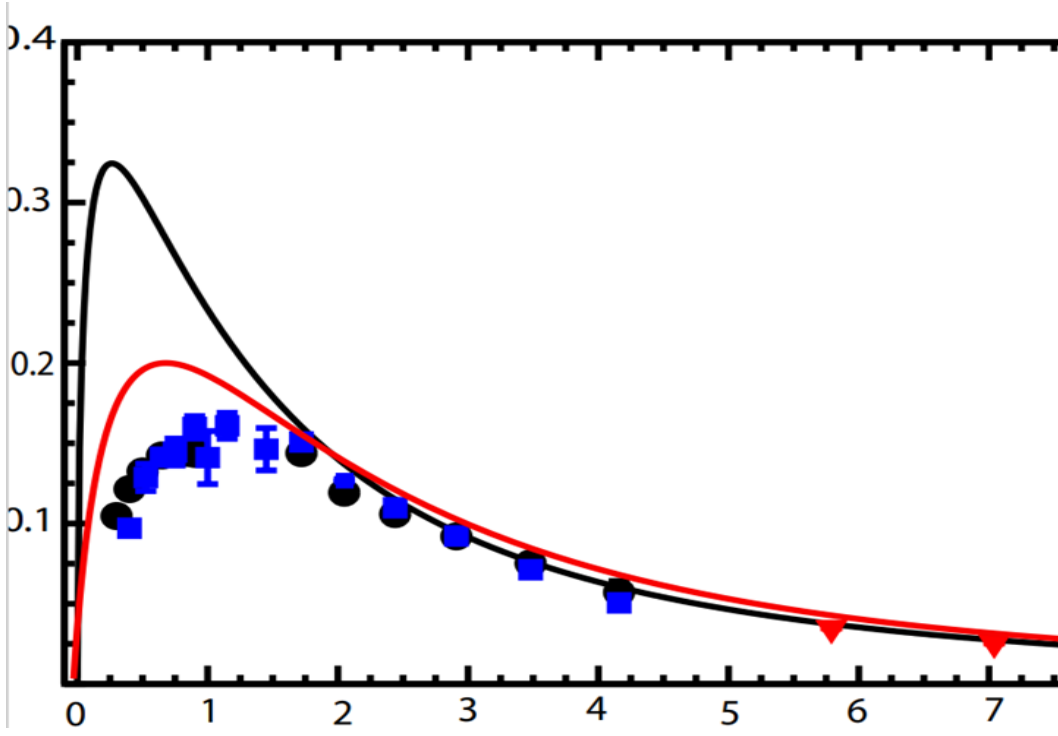
FIG. 1: Results for the N + \gamma^* \rightarrow R(1535) transition Dirac form factor obtained by the hard-wall model (red thick solid line), given by the semirelativistic approximation (black thick solid line) [17]. Data from CLAS [13] (full circles), MAID [14,15] (full squares), JLab/Hall C [16] (triangles).
