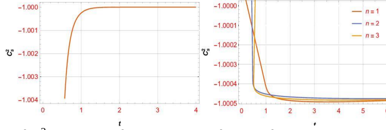
Figure 3. The plot of C_s^2 in terms of t and n = 2 in fig (3a) for model I and in fig (3b) for model II, according to the different values of n and constant parameters \alpha = \beta = 0.1
