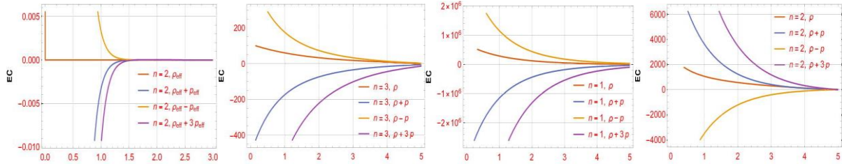
Figure 2. The plot of EC in terms of t in fig (2a) for model I and in fig (2b, 2c, 2d) for model II, according to the different values of n and constant parameters \alpha = \beta = 0.1 , \lambda = 1.5 , \delta = 1
