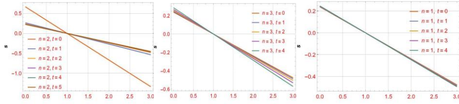
Figure 4. The plot of \dot{s} in terms of \dot{r} in fig (4a) for model I and in fig (4b,4c) for model II, according to the constant parameters \alpha = \beta = 0.1 , \lambda = 1.5 and \delta = 1
