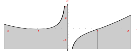
Figure 1: The allowable area indicates the particles' energy E and spins s to reach the event horizon, and particles with the highest energy spin of -0.6 < s < 0 .
