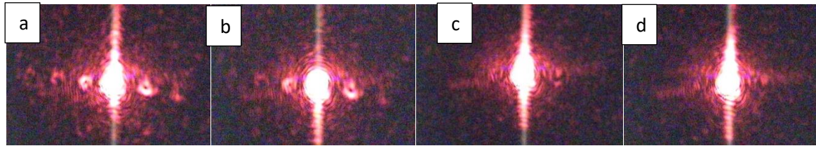
Figure 4: diffraction order of DDLC by applying electric field a) v=1.72\text{V} b) v=2.59\text{V} c) 14.1\text{V} d) 22.1\text{V}
